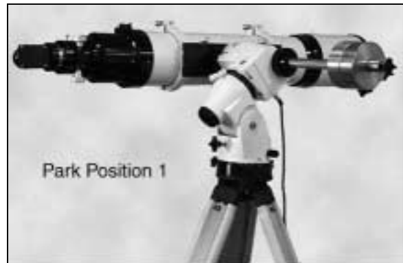
Scope is level and pointing north. This position is also called the Reference Park Position. RA horizontal, Dec = 90 - Latitude
